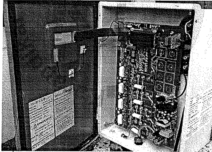
Picture2 : No ingress of powder & water observed
